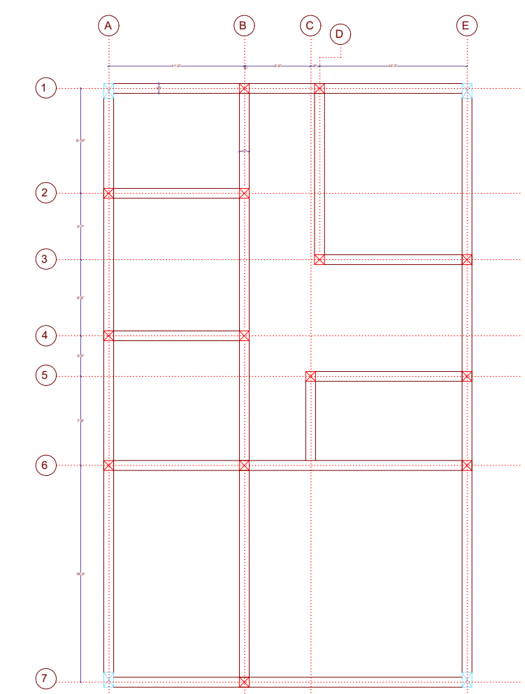
BEAM LAYOUT OF GROUND FL.
