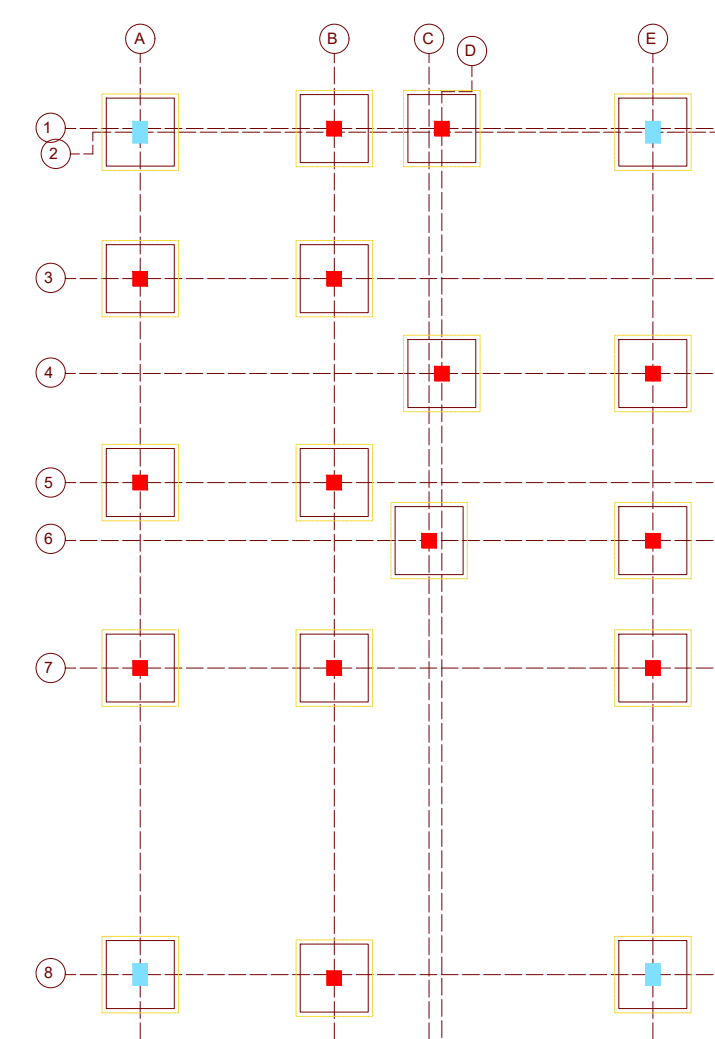
FOOTING LAYOUT WITHOUT SLAB
