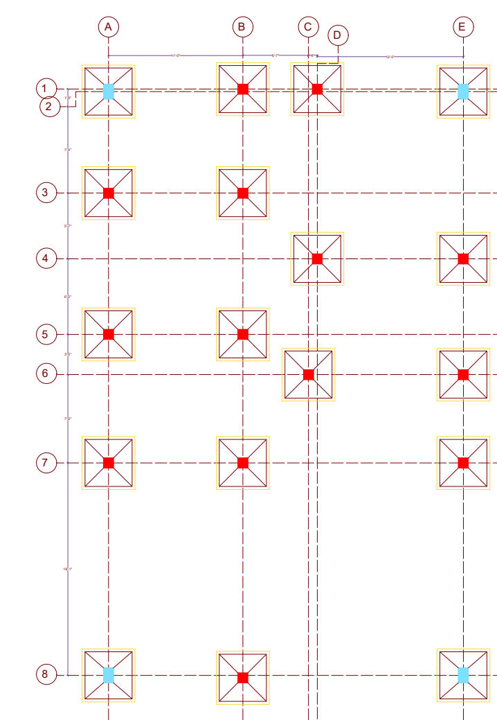
FOOTING LAYOUT WITH SLAB
